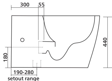
(Optional connector setout range 75-215 mm)
